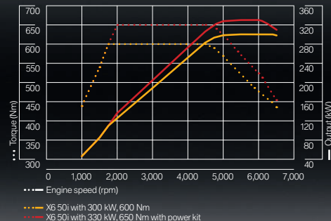
Performance data for BMW X6 50i with BMW Performance power kit Full-load performance of X6 50i
