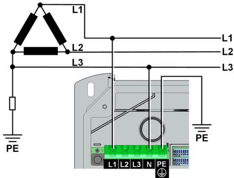
Connection to a three-wire IT system
