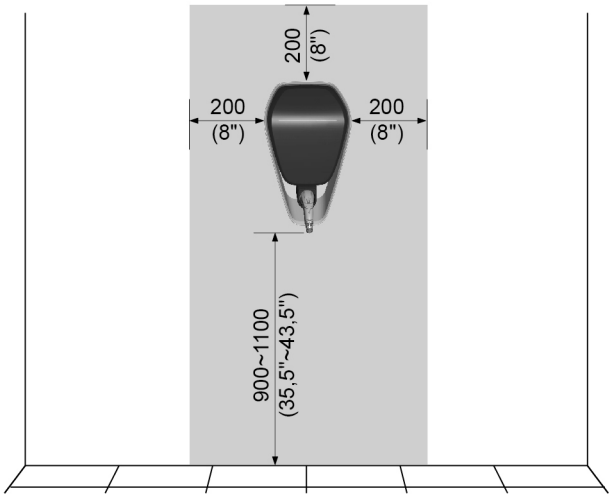
Dimensions in millimetres (inches)
